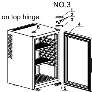
1.Hinge Cover 2.M5X12 Screw 3.Top Hinge 4.Door 5.Bottom hinge 6.Screw cap
