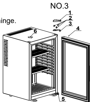
1.Hinge Cover 2.M5X12 Screw 3.Top Hinge 4.Door 5.Bottom hinge 6.Screw cap
